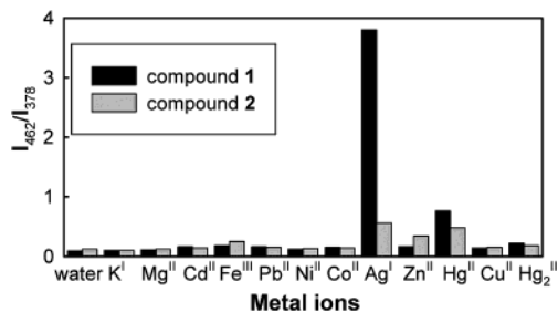
Figure 3. The responses of compounds 1 (black) and 2 (gray) to metal solutions (150 \mu\text{M} , x-axis markers). Excitation was at 344 nm, and emission was at 462 and 378 nm.
