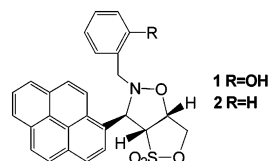
Figure 1. Drawing of fluorescent sensor 1 and analogue compound 2 .
