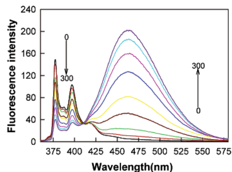
Figure 2. Fluorescence emission spectra of 1 in the presence of different concentrations of Ag I (0, 4.0, 10, 15, 20, 40, 75, 150, 300 μM). Excitation wavelength was 344 nm. The concentration of 1 was 0.8 mM.
