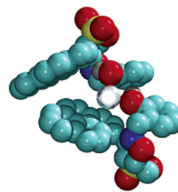
Figure 4. A proposed structure for compound 1 + metal ion.
